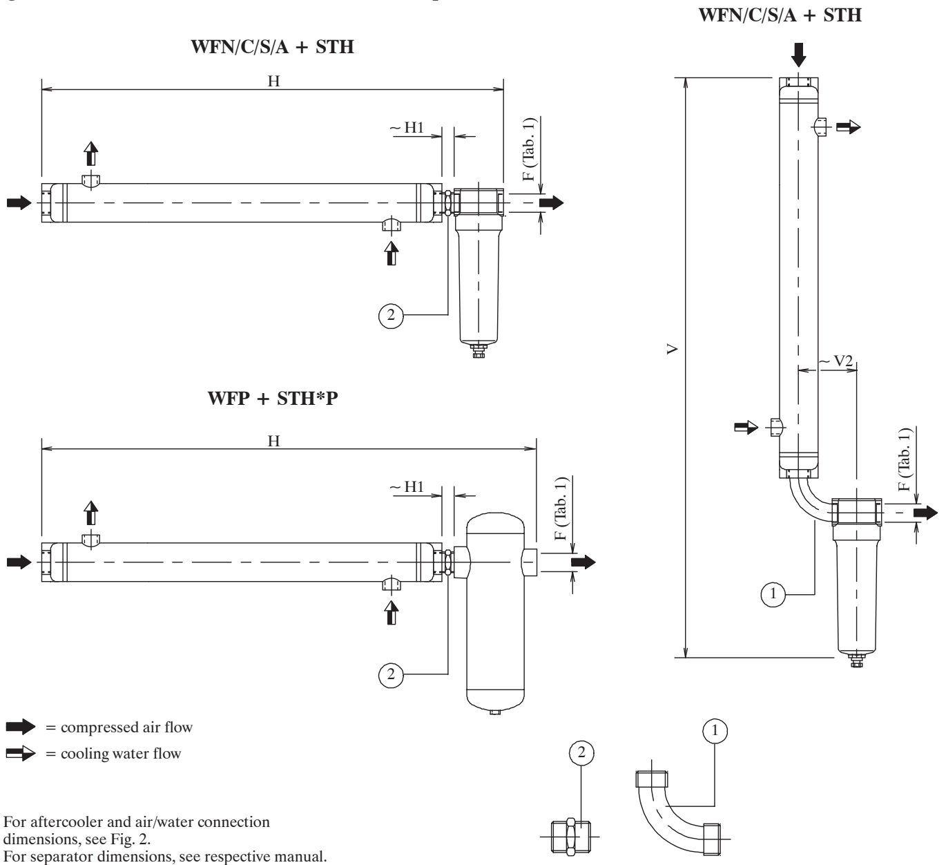
Fig. 3 – Combined Aftercooler (WF*001–013) + Separator (STH)
