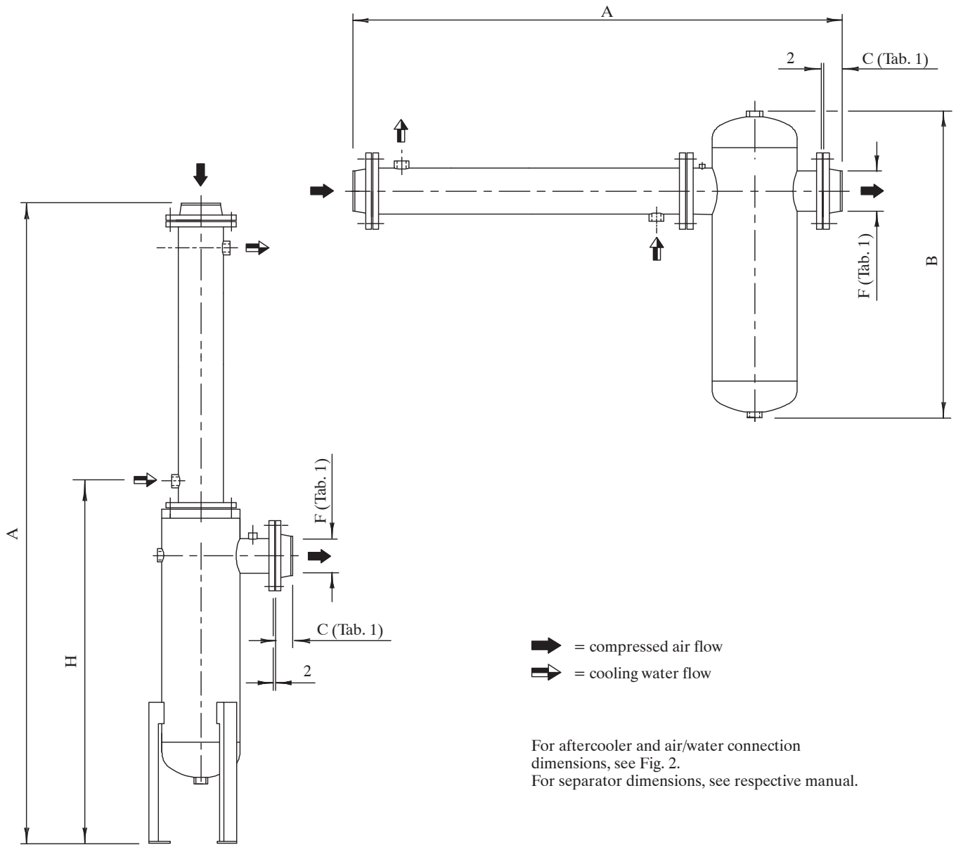
Fig. 4 – Combined Aftercooler (WF*016–090) + Separator (SFH/SFV)
